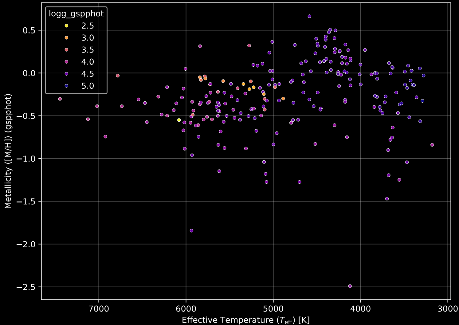
APOGEE DR17 Field: [K2_C1_254+62_btx] Stellar Population Parameters (n= 225)
